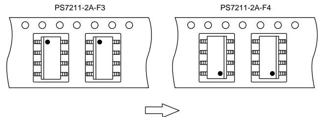
TAPE DIRECTION
